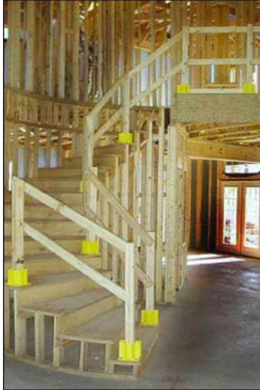
Figure 33 - Wooden guardrail system for a stairway.
